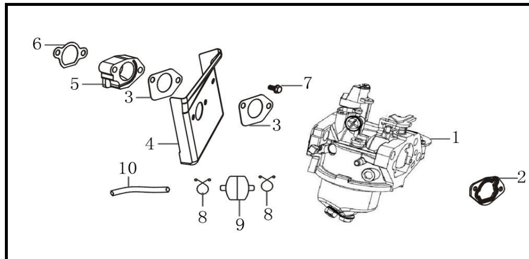
Carburetor With Pump
